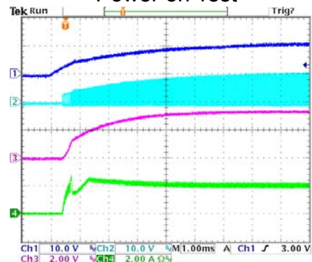
Ch1: V IN , Ch2: LX, Ch3: V OUT , Ch4: I LX
